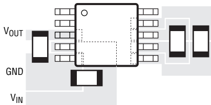
Figure 6. Recommended Layout
